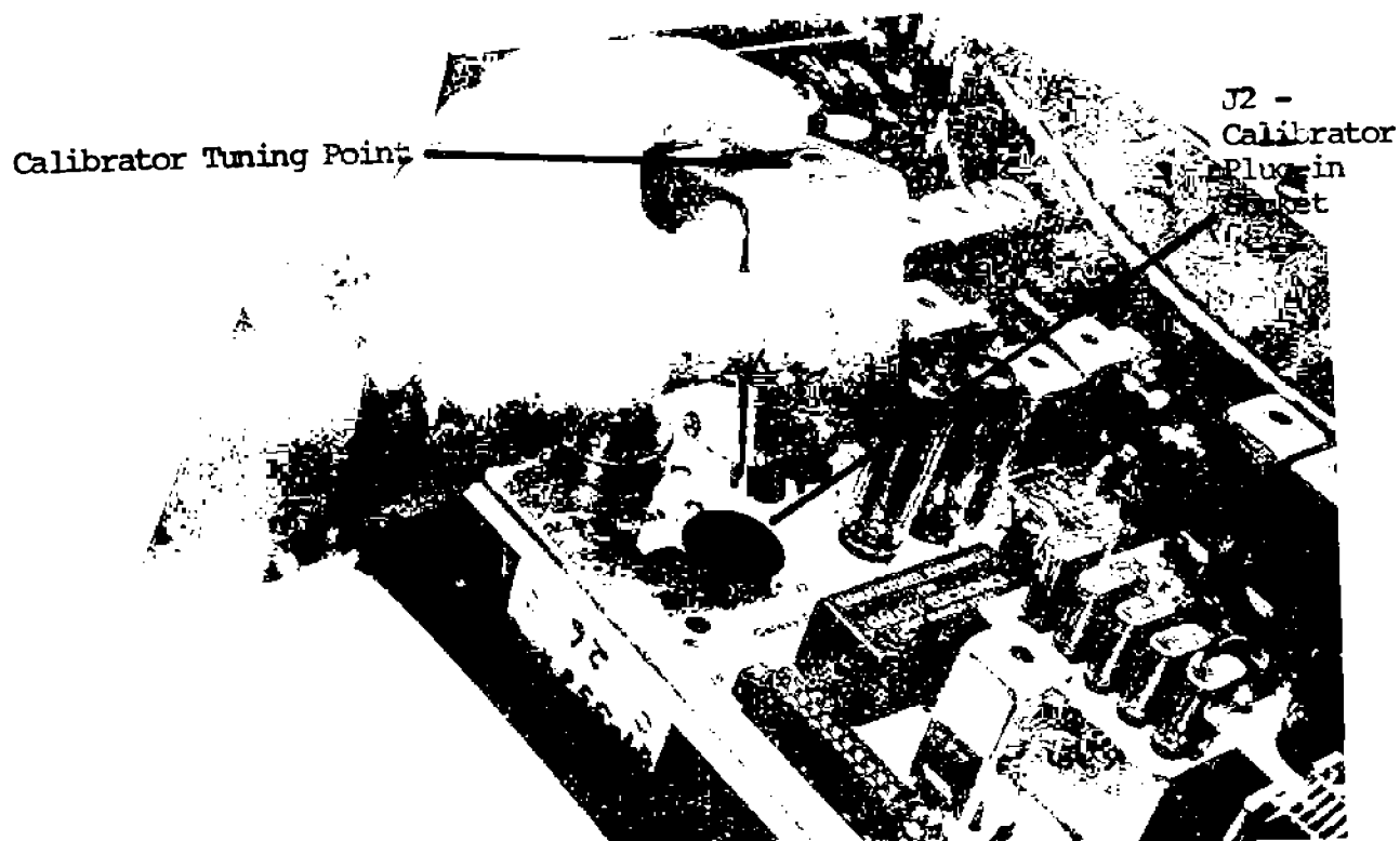
CALIBRATOR INSTALLATION
