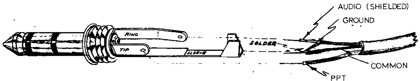
MICROPHONE CONNECTION
