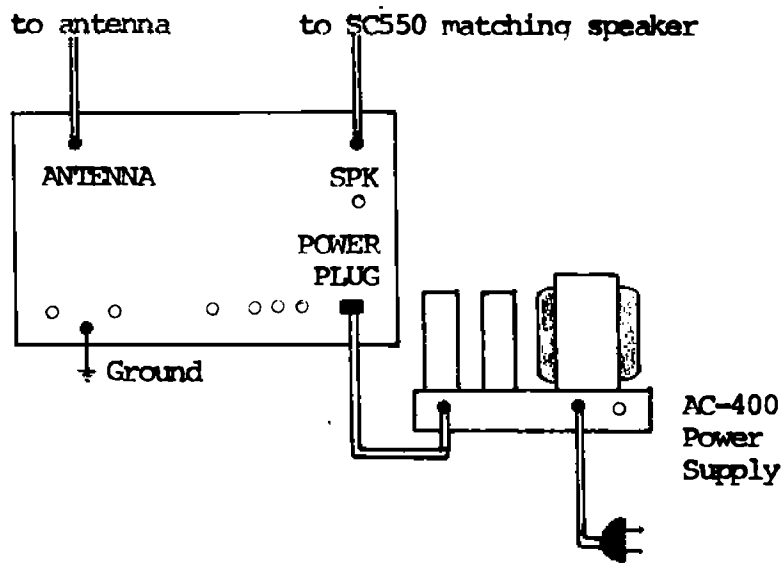
FIXED STATION CABLE CONNECTIONS FIGURE 3
